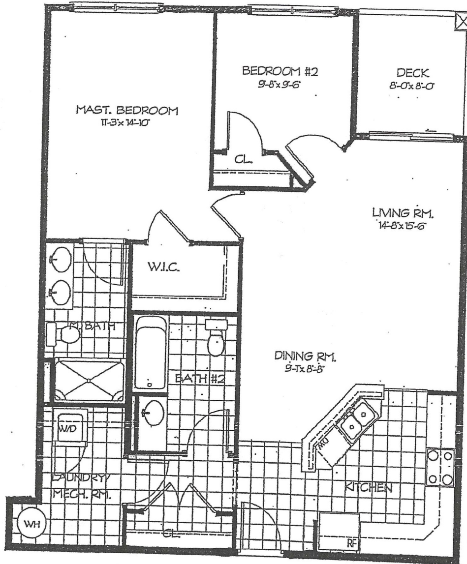
2 - BEDROOM UNIT MODEL "C" 1,034 SQ. FT. SCALE: 1/8" = 1'-0"
